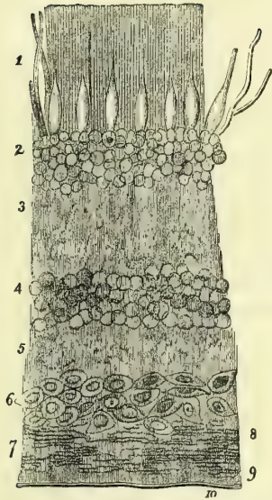
Vertical Section of Retina of the Human Eye.
